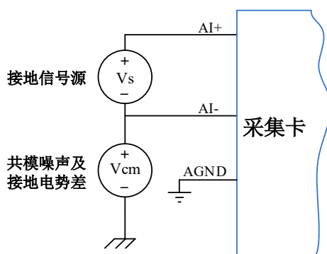
图 4-5-5 接地信号源的差分 (DIFF) 连接
